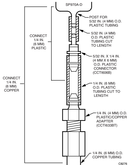
Fig. 5. Adaptation piping.
